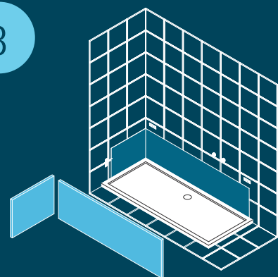
3. FISSAGGIO COPERTURE A MURO 3. FIXING OF COVER PANELS
