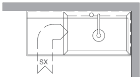
IN NICCHIA SINISTRA ENTRY AT LEFT IN NICHE INSTALLATION
